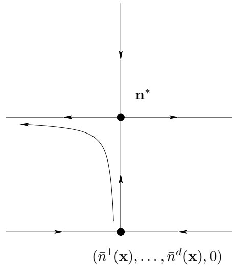
Figure 2.4: Assumption (B1) prevents such situation.
