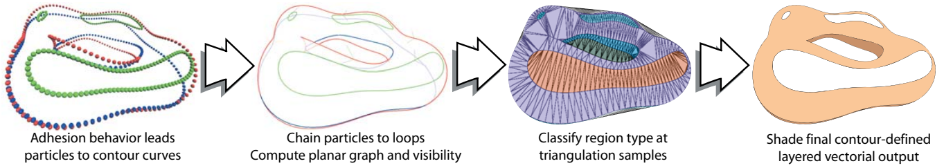
Fig. 14. We convert an implicit surface specified by a function into clipart specified by layered filled 2-D polygons by using particles to find surface feature curves and determining how those closed spacecurves should be layered and shaded when projected to 2-D.
