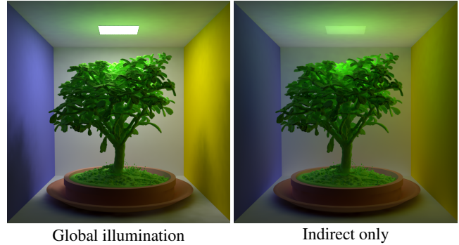
Figure 6: A scene containing various surface representations, rendered with a meshless hierarchical radiosity plugin to PBRT. The box is a mesh, the bonsai is an isosurface from a volumetric dataset and the pot is made out of implicit surfaces.
