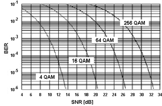
Figure 1: SNR versus BER for different QAM schemes
