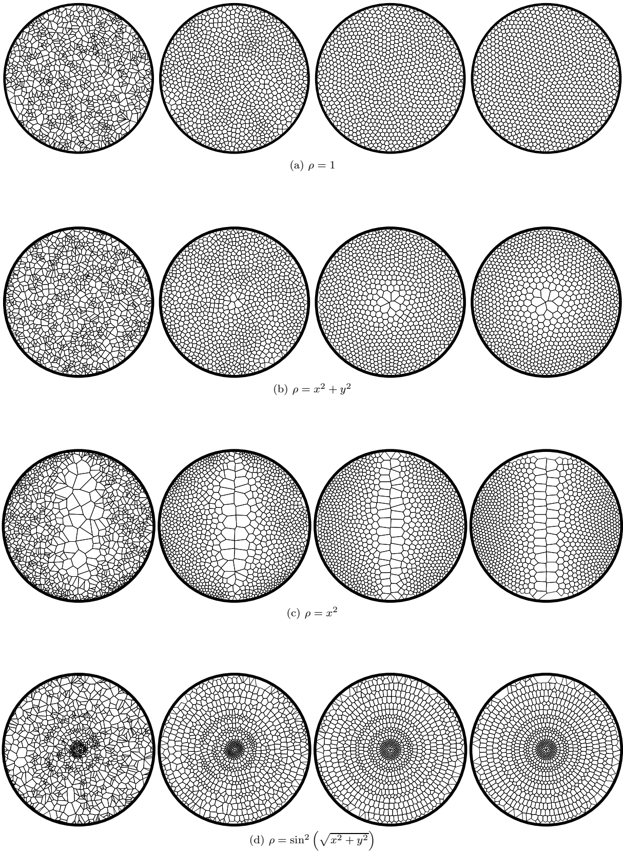
Figure 3: Each column correspond to the 1st, 10th, 100th and 1000th iteration.
