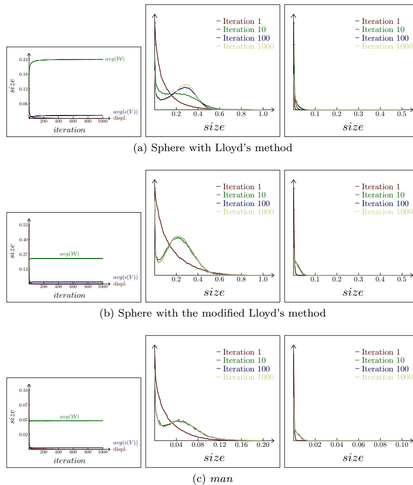
Figure 6: In the first column, the corresponding avg(\mathcal{W}) and avg(\epsilon(V)) versus displacement size graph. In the second column, we have the distributions for \mathcal{W} and avg(\epsilon(V)) on the iterations 1, 10, 100 and 1000 respectively. Remark: in (c), the size goes from 0 to 0.2 because points in man have a sparse distribution in the volume of reference.
