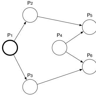
Figure 3: Network considered in Theorem 2
