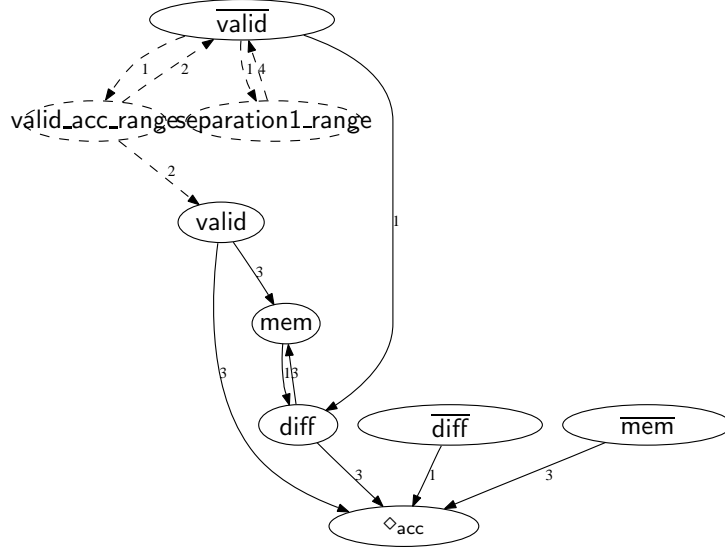
Figure 5: Dependency Graph of Axiom (1), with Post-Fixed Comparison Predicates and Some Vertices and Arcs From Other Axioms
