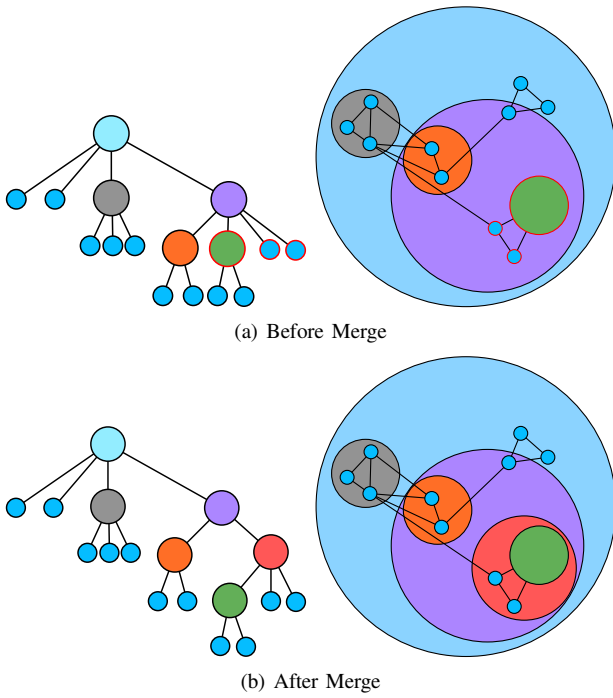
Fig. 7. A merge operation example. Selected nodes in (a) are grouped into a single metanode at the current level of the hierarchy as shown in (b). For a merge operation, the selection cannot cross open metanode boundaries.
