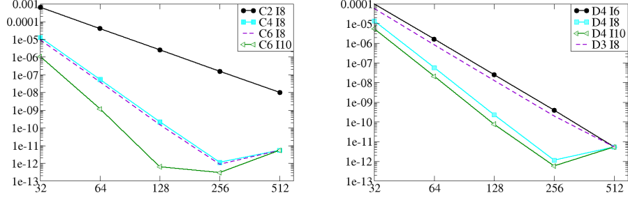
Figure 6: Harmonic Oscillator, {}^2\tau_p as a function of 2^J , for different orthogonal bases m_1 : Coiflets (left) and Daubechies (right). The curves C6I10 and D4I10 show the influence of m_2 on the convergence.
