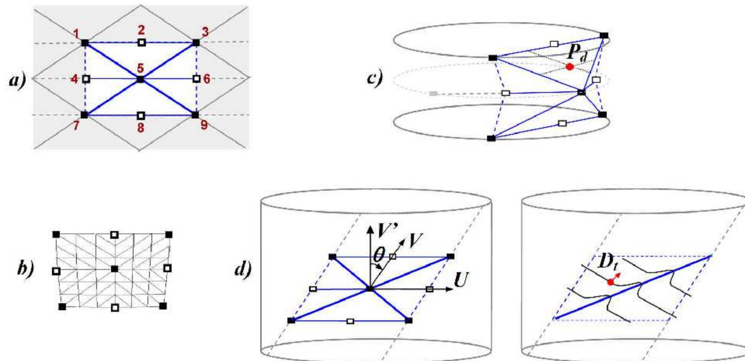
Figure 8: (a) Buckling patch made of 9 control points that guide the procedural deformation. (b) Refined mesh interpolating the control points. (c) Transformed triangles of a diamond buckling pattern. (d) Fold across the selected diagonal of a twist buckling pattern.
