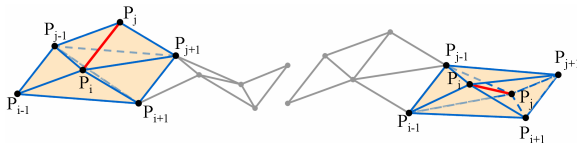
Figure 2: Locally convex (left) and non-convex (right) interior triangulation edges P_i P_j .
