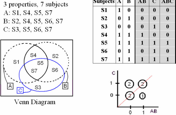
Figure 2: Extraction of AB \rightarrow C from data.
