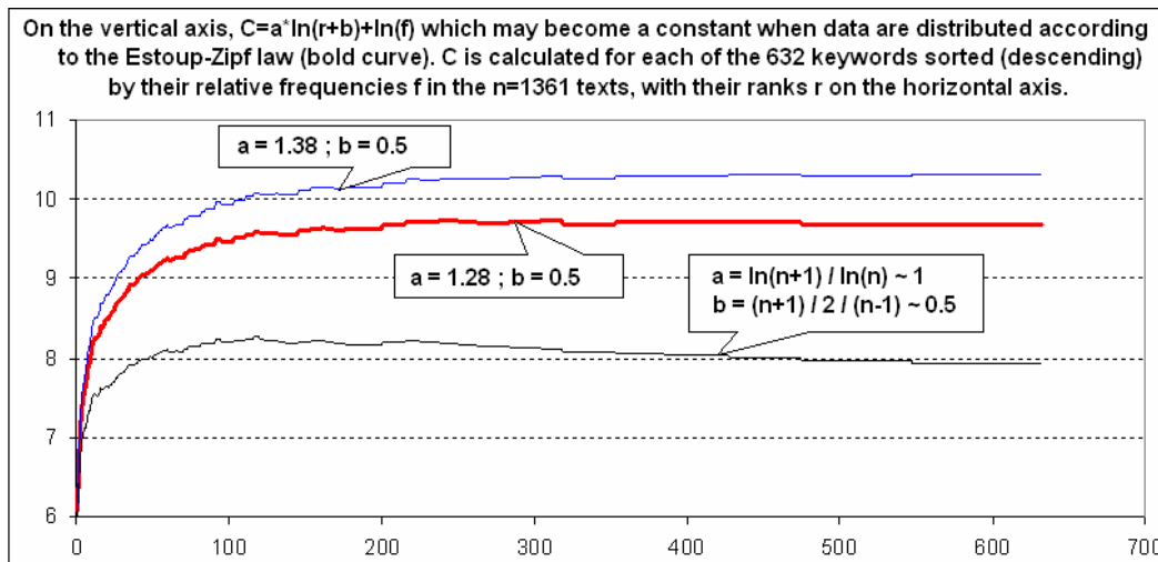
Figure 4 : Bringing out the parameters ( a=1.28 and b=0.5 ) of the “Zipf-like” law of the corpus of texts.
