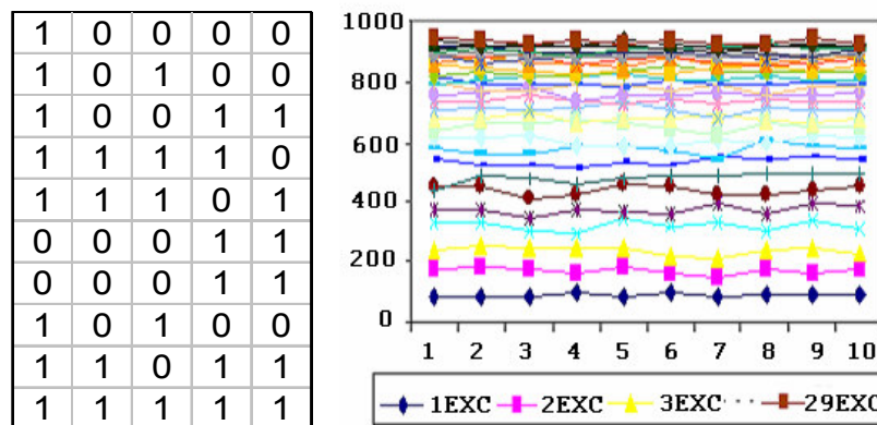
Figure 11: Results obtained for data on the left for 10 trial runs of 1000 simulations with a number of exchanges between 1 to 29.
