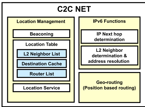
Fig. 4. Functional block
