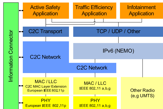
Fig. 1. C2C-CC Architecture
