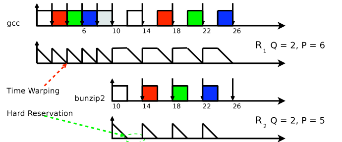
Figure 3: IRIS solves the deadline aging problem by having VRESes wait until the next deadline before replenishing their budget. The replenishment can be instantaneous due to time warping.
