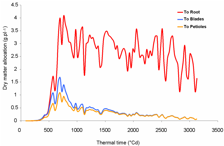
Fig. 9 Biomass allocation between blade, petiole and root compartments simulated by the GreenLab model
