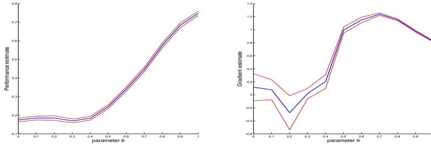
FIG. 2 – Left : Performance estimation \frac{1}{M} \sum_{m=1}^M J_{\omega_m}^N(\theta) (bold curve) of J(\theta) and confidence intervals \pm \sqrt{\text{Var}[J_{\omega}^N(\theta)]/M} . Right : Gradient estimation \frac{1}{M} \sum_{m=1}^M \partial_h J_{\omega_m}^N(\theta) of \partial J(\theta) and confidence intervals \pm \sqrt{\text{Var}[\partial_h J_{\omega}^N(\theta)]/M} .
