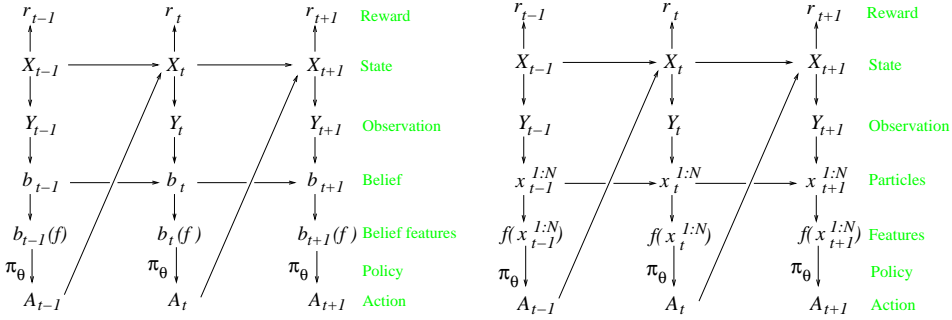
FIG. 1 – Left figure : Causal and temporal dependencies in a POMDP. Right figure : PF-based scheme for POMDPs where the belief feature b_t(f) is approximated by \frac{1}{N} \sum_{i=1}^N f(x_t^i) .
