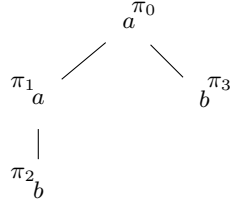
(a) A tree t \in T_{\{a,b\}}
