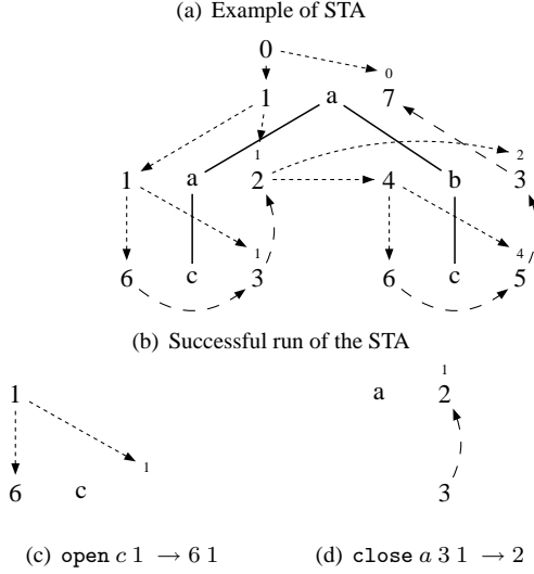
Figure 2. An STA, and an example of run
