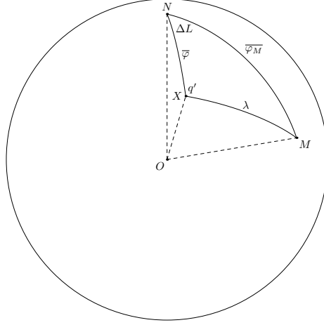
Figure 1: The problem of the Qibla at location X : M is the Mecca, N is the North pole and O is the center of the Earth. \varphi_M and \varphi are the latitudes of Mecca and of X . \overline{\varphi}_M = 90^\circ - \varphi_M and \overline{\varphi} = 90^\circ - \varphi are the colatitudes of Mecca and X . The difference of longitudes L_M and L is \Delta L . Then q' (measured from North) or q = 180^\circ - q' (measured from South) is the qibla angle.
