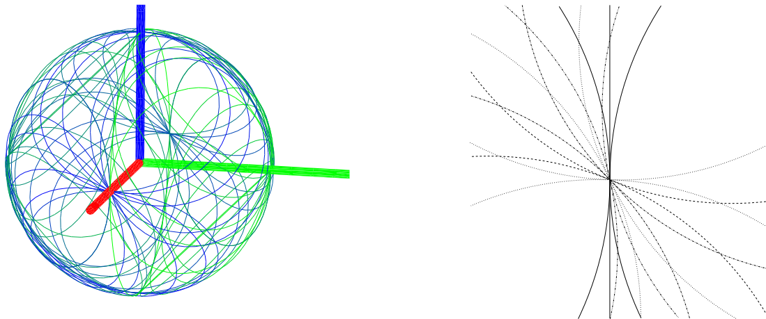
Figure 5: Left: degenerate arrangement of 47 circles on S_0 . Right: zoom about the point (r_0, 0, 0) : six different directions of tangency for thirteen circles. This point is a \theta -extremal point for two circles. Ten circles (two among them being polar) intersect at that point and a bipolar circle passes through it. This arrangement features 674 vertices, 1384 edges, 712 faces and no holes. Euler characteristic reads as 674 - 1384 + 712 = 2 .
