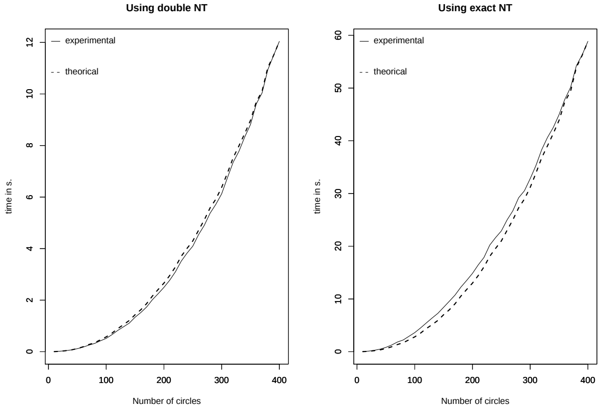
Figure 4: Observed vs theoretical complexities for random arrangements.
