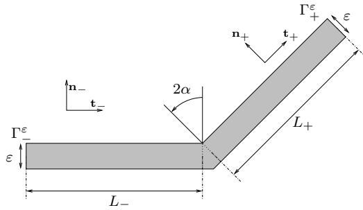
Figure 1.1: Configuration of the domain \Omega_\alpha^\varepsilon
