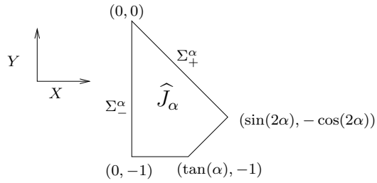
Figure 1.2: The normalized junction \hat{J}_\alpha
