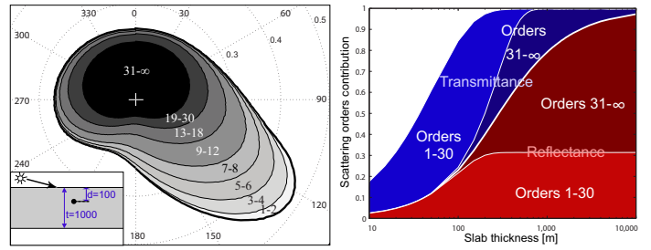
Figure 3: Some results of our light transport analysis. Left: BSDF for a point of view at a depth d = 100m inside a cloud slab of thickness t = 1000m , with an incident illumination angle \phi_L = 75^\circ . Areas represent the contribution of different orders of scattering. Even high orders (up to 30 scattering events) show an anisotropic behavior, while orders > 30 show an isotropic behavior. Right: Contribution of different orders of scattering for the reflectance (in red) and transmittance (in blue) of a slab of varying thickness. Isotropic orders (31- \infty ) begin to appear at thicknesses > 100m . Anisotropic orders (1-30) play a role up to 1000m in transmittance and contribute to 30% – 100% of the reflectance.
