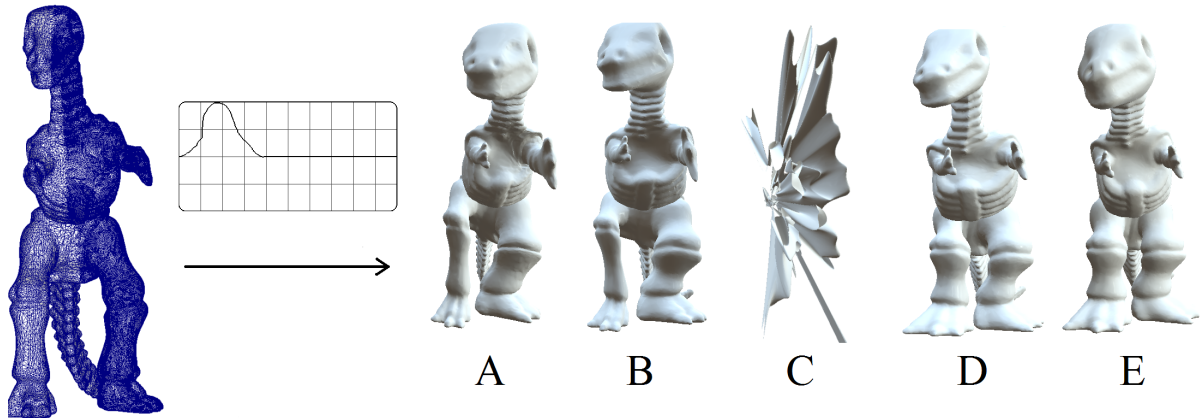
Figure 2: Filtering an irregularly sampled surface (twice denser on the right half) with different discrete laplacians. Combinatorial Laplacian (A), unweighted cotan \cot(\beta_{ij}) + \cot(\beta'_{ij}) (B) and symmetrized weighted cotan (\cot(\beta_{ij}) + \cot(\beta'_{ij})) / (A_i + A_j) (D) produce deformed results (right leg is bigger). Weighted cotan (\cot(\beta_{ij}) + \cot(\beta'_{ij})) / A_i are not symmetric which does not allow for correct reconstruction (C). Only our symmetric weights (\cot(\beta_{ij}) + \cot(\beta'_{ij})) / \sqrt{A_i A_j} are fully mesh-independent (E).
