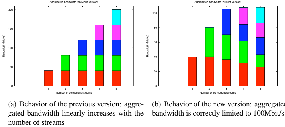
Figure 3: Inter-islet aggregated bandwidth when adding streams (shown in different colors). Node bandwidth: 40 Mbit/s, Inter-islet link: 100 Mbit/s.
