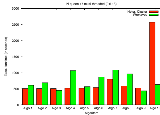
Figure 10: Computation time of the different algorithms for the N -queen problem of size 17, using the heterogeneous cluster or Wrekavoc, multi-threaded version, kernel 2.6.18
