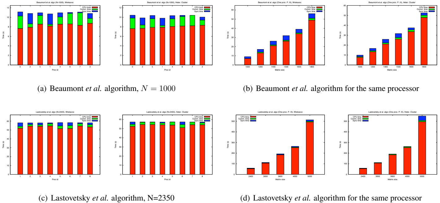
Figure 7: Comparison of node runtime (CPU, communication and synchronization) for the static load balancing application
