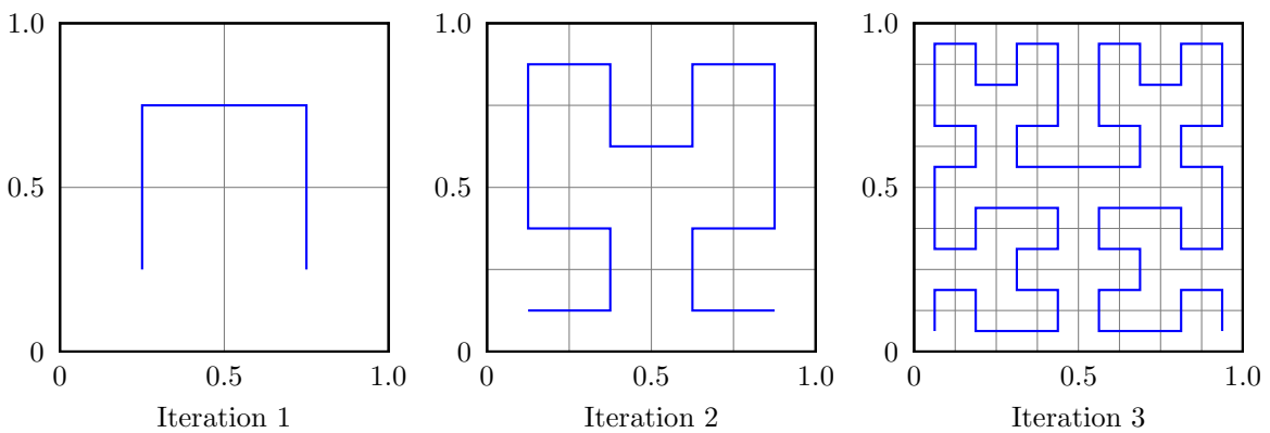
Figure 3.3: Recursive construction principle of the two dimensional Hilbert curve.
