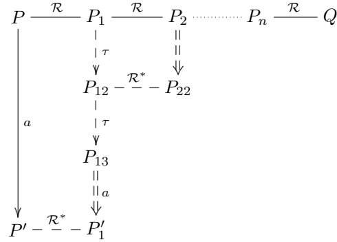
Figure 4: Compatible refinement for HO \pi P
