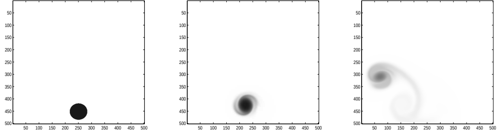
Figure 2: Concentration images extracted from a simulation of a shallow water model coupled with a concentration equation, images number 1 (left), 101 (middle), and 401 (right) respectively.
