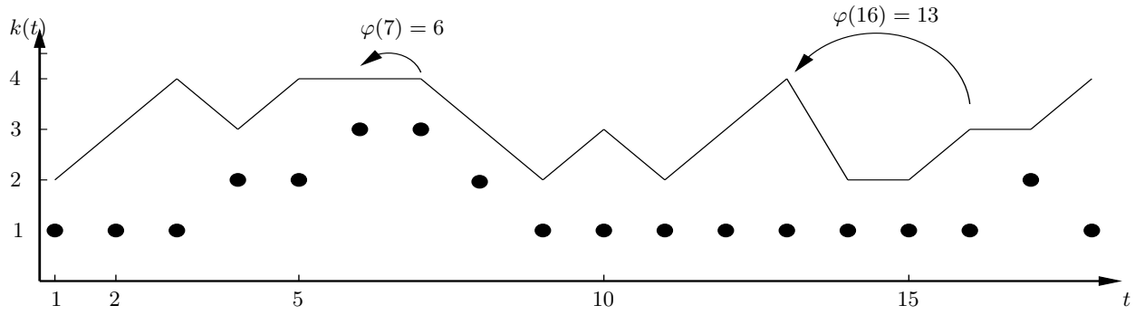
Fig. 6. A possible curve for \kappa(t) , with the corresponding values for \alpha(t)
