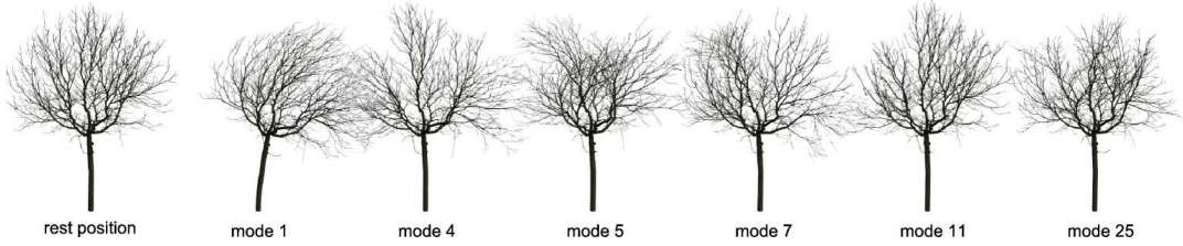
Figure 4: The modes of deformation of the walnut model. During animation the final displacement of a tree is a combination of its modal deformation. The modes are sorted in ascending order of their natural frequencies.
