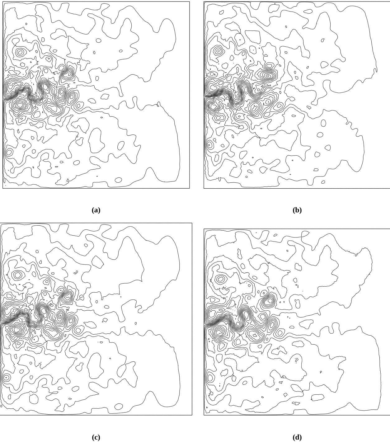
Fig. 12. Upper layer of: true initial state (a) , initialization (or background) state for both 4D-VAR and BFN algorithms (b) , and initial states identified by the BFN (c) and 4D-VAR (d) algorithms.
