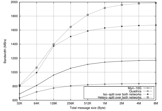
Fig. 8. Message splitting - Bandwidth
