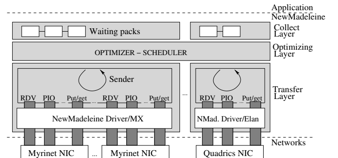
Fig. 5. NewMadeleine architecture.
