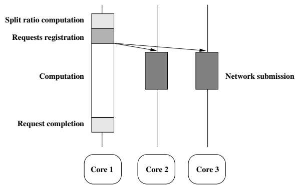
Fig. 7. Sending eager packets over parallel networks
