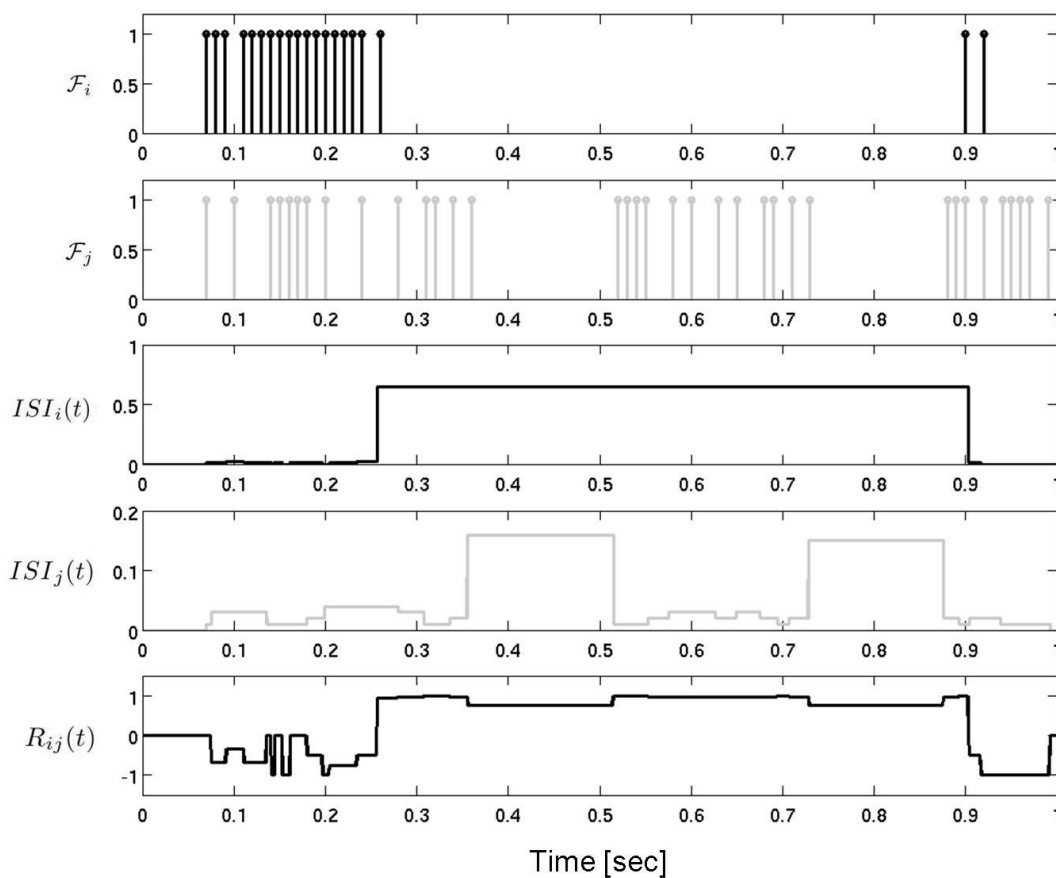
Figure 11: Synchrony between the spike trains of a pair of neurons. \mathcal{F}_i and \mathcal{F}_j are the spike trains of MT neurons i and j , respectively. The respective ISI representations defined in (13) are shown as ISI_i(t) and ISI_j(t) . Finally, the ratio between ISI_i(t) and ISI_j(t) is shown as R_{ij}(t) .
