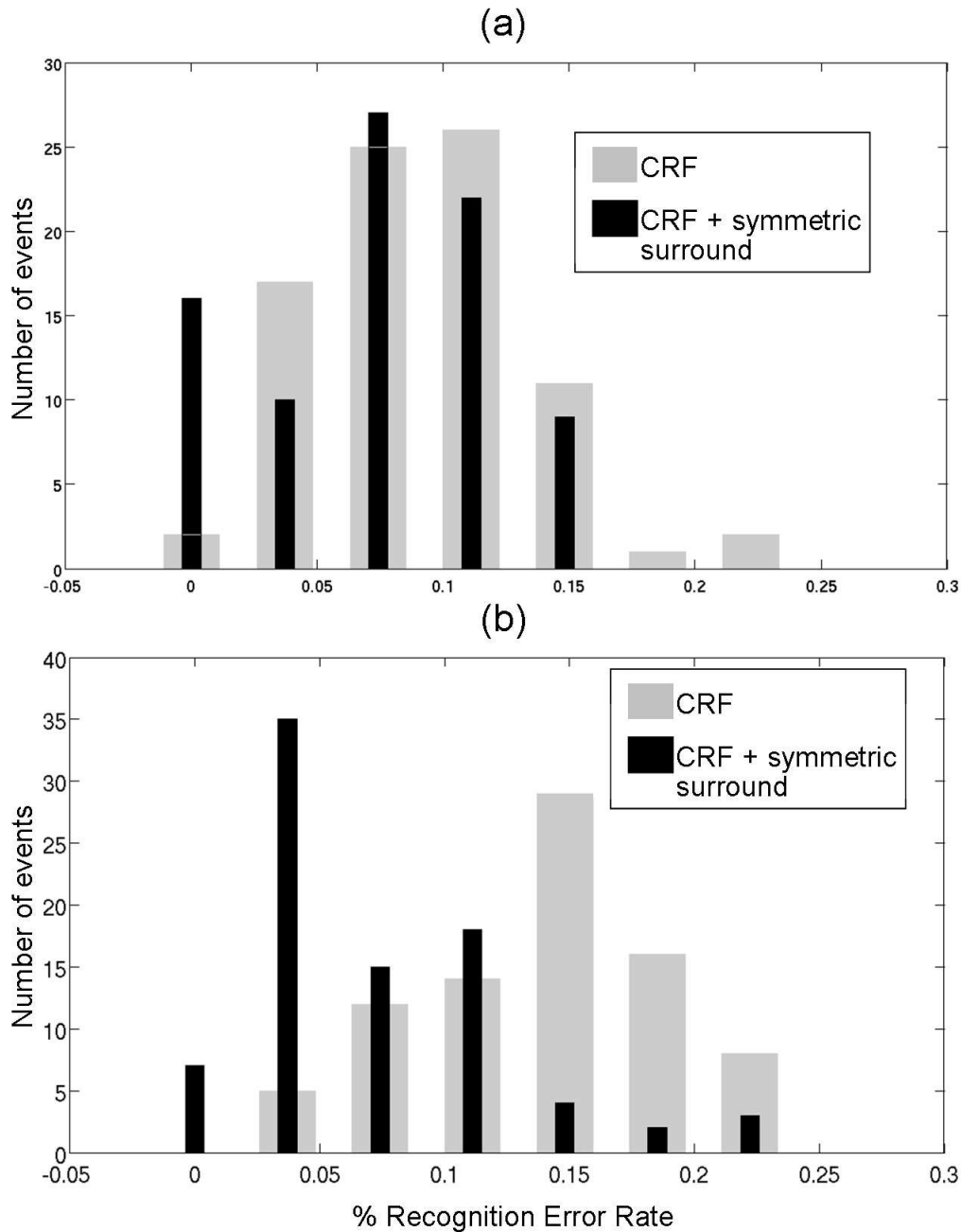
Figure 14: Histograms representing the recognition error rates obtained by our approach in Weizmann database, using: MT CRFs (gray bars) and MT center-surround interactions shown in Figure 9 (black bars). The results were obtained using the 84 possible training sets built with 6 different subjects. (a) Histogram obtained for mean motion maps . (b) Histogram obtained using synchrony motion maps .
