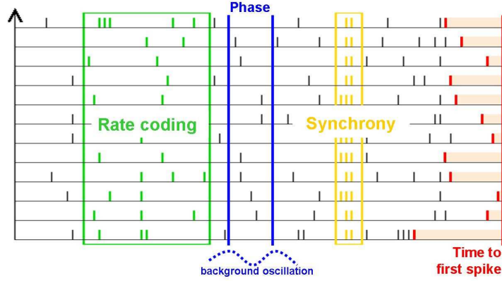
Figure 1: Example of a raster plot and illustration of some different methods to analyze the neural code (see text for more details). Each horizontal line can be interpreted as an axon in which we see spikes traveling (from left to right).
