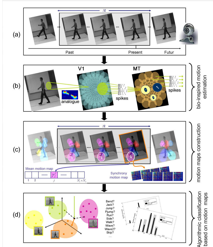
Figure 3: Block diagram showing the different steps of our approach from the input image sequence as stimulus until its final classification. (a) We use real video sequence as input, the input sequences are preprocessed in order to have contrast normalization and centered moving stimuli. To compute the motion maps representing the input image we consider a sliding temporal window of length \Delta t . (b) Directional-selectivity filters are applied over each frame of the input sequence in a log-polar distribution grid obtaining spike trains as V1 output. These spike train feed the spiking MT which integrates the information in space and time. (c) The motion maps ( mean motion map and synchrony motion map ) are constructed calculating either the mean firing rates of MT spike trains or a synchrony map of the spikes trains generated by MT cells. Both motion maps are created considering the spike trains inside the sliding temporal window of length \Delta t . (d) Classification stage where, starting from the motion maps and the training set content, a final action is assigned to the input image sequence..
