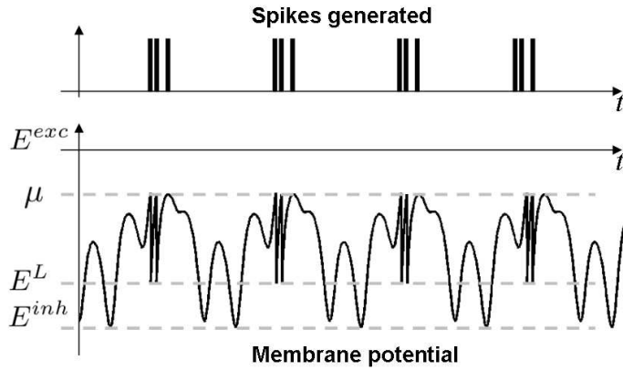
Figure 2: Temporal evolution of the membrane potential of a neuron and its corresponding spikes generated. A spike is generated when the membrane potential exceeds the threshold \mu ( E^L < \mu < E^{exc} ). When the spike is emitted membrane potential returns to its resting value E^L .
