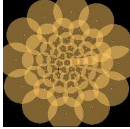
Figure 6: Sample of log-polar architecture used for a MT layer. The cell distribution law is divided into two zones, a homogeneous distribution in the center with a certain radius and then a periphery where the density of cells decays with the eccentricity.
