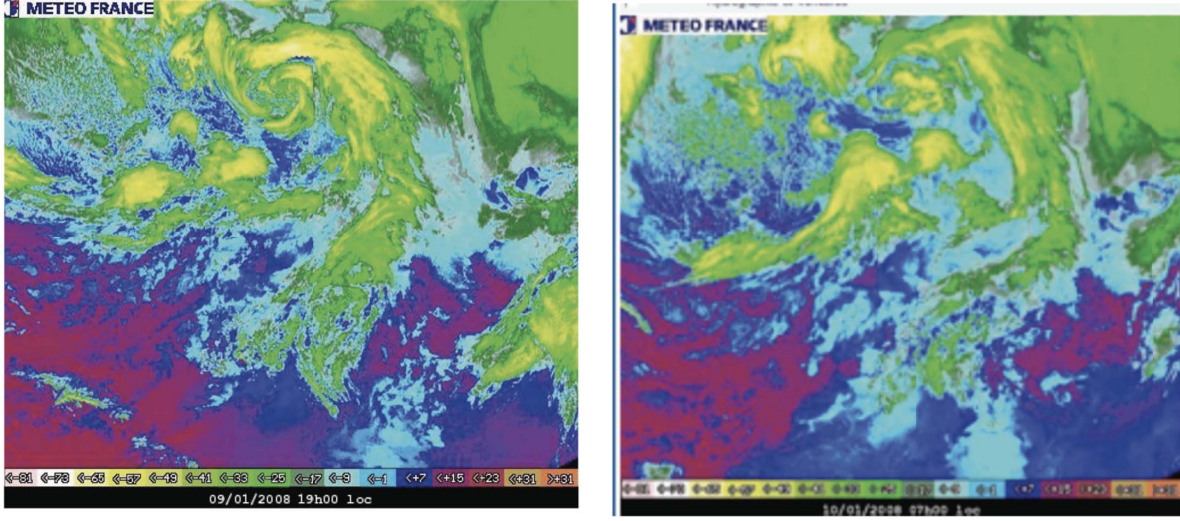
Fig.8 (left) Europe on 09/01/08 at 19:00 on infrared channel (source MétéoFrance) Fig.9 (right) Europe on 10/01/08 at 07:00 on infrared channel (source MétéoFrance)
