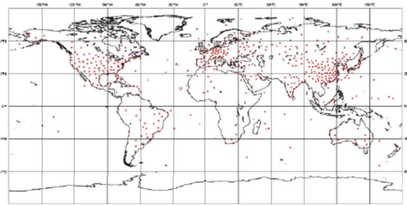
Fig.2 Wind, temperature, specific humidity
