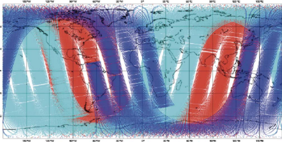
Fig.3 Polar orbiting satellites
