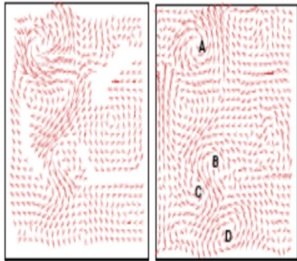
Fig.11 Estimated (left) and actual fields
