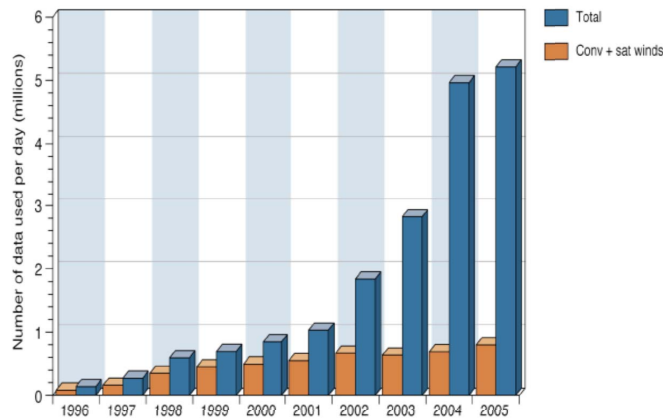
Fig.5 Total number of observations per days (source ECMWF)
