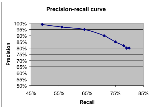
Figure 3: Precision-recall curve in our first person "global" re-identification experiment
