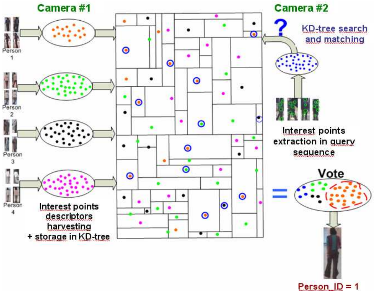
Figure 1: schematic view of model building (left), and of re-identification of a query (right).
