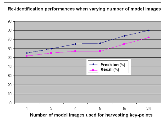
Figure 4: Influence of the number of images used per model on the re-identification precision and recall
