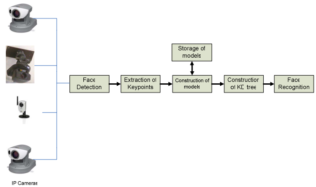
Figure 6: The general diagram of our application to real-time on-the-fly face identification
