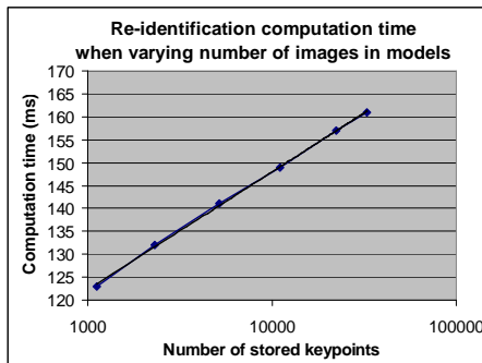
Figure 5: Re-identification computation time as a function of number of stored keypoint descriptors; the dependence is clearly logarithmic
