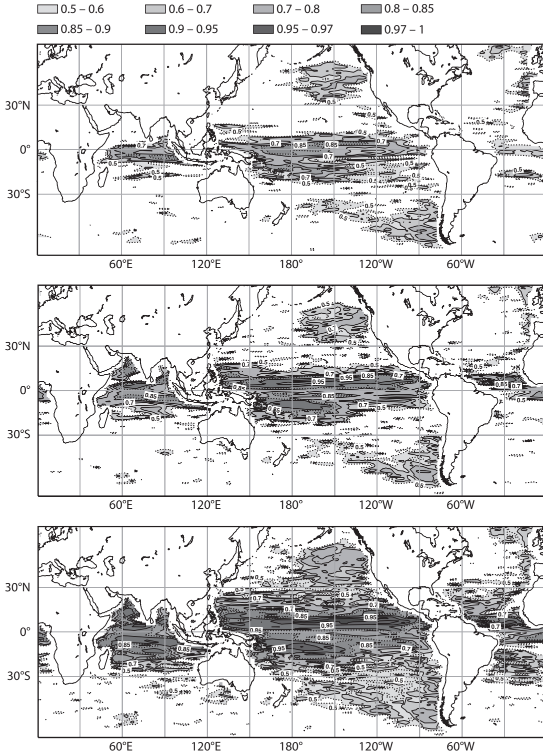
Fig. 11: Correlations with Oscar zonal component of the surface currents for Control (top), ETS (middle) and E_TSA_dTr (bottom)
