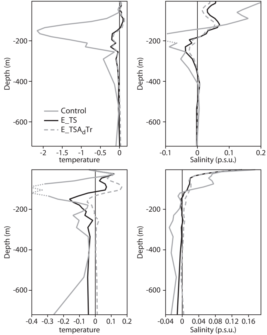
Fig. 10: Mean Analysis minus Observation averaged over the NINO4 (top) and Tropical Atlantic (bottom) regions for temperature (left) and salinity (right) for Control (grey), E TS (black) and E TSA d Tr (dashed grey)
