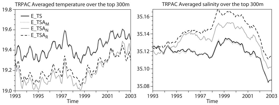
Fig. 5: Time series of temperatures (left) and salinity (right) averaged over the tropical Pacific ( [30S, 30N] ) and the first 300 meters of the experiments E_{TSA_M} (dotted), E_{TSA_N} (grey), E_{TSA_R} (dashed) and E_{TS} (black).
