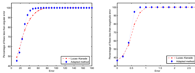
Fig. 10. Relative performance of the two algorithms with sequence :rotation around Z-axis of 1. Left: percentage on angle error. Right: magnitude of difference performance
