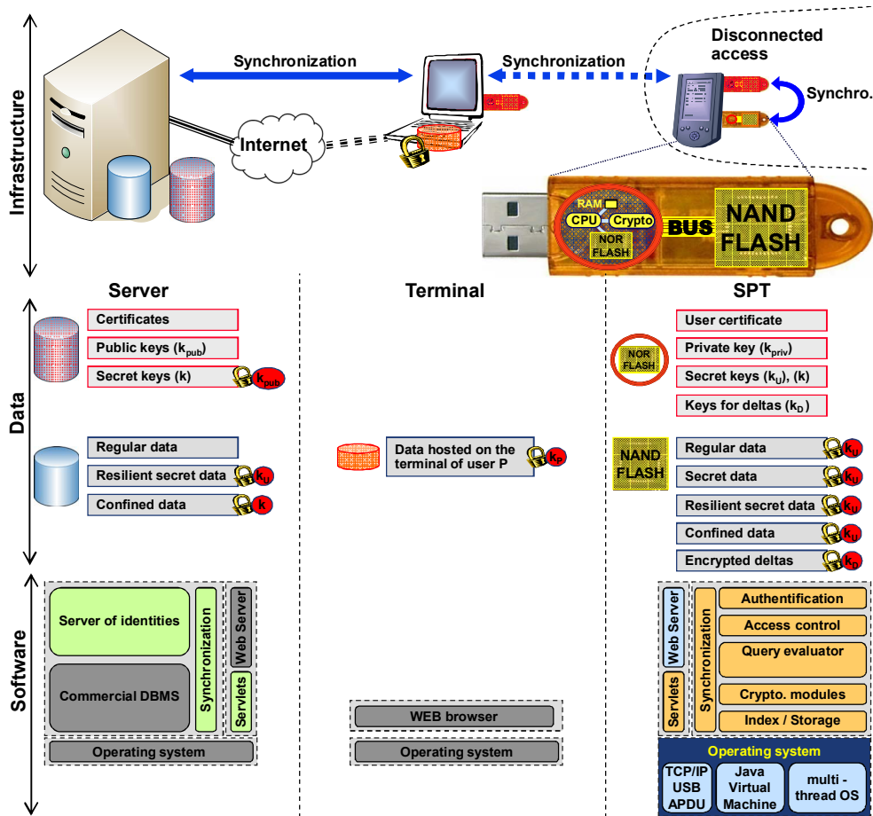
Figure 1: Functional architecture
