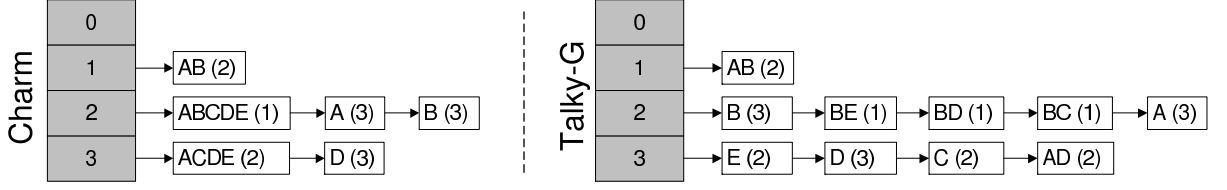
Figure 3.1: Hash tables for dataset \mathcal{D} (Table 2.1) by \min\_supp = 1 . Left: hash table of Charm containing all FCIs. Right: hash table of Talky-G containing all FGs.
