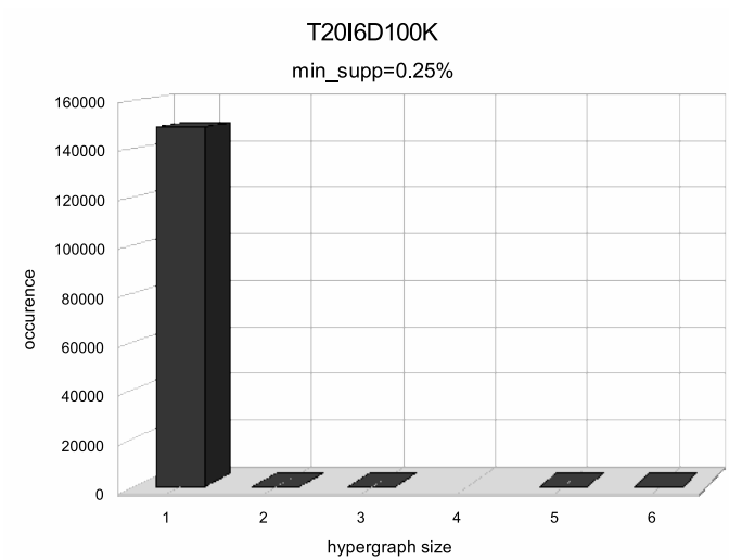
Figure 4.3: Distribution of hypergraph sizes for T20I6D100K.
