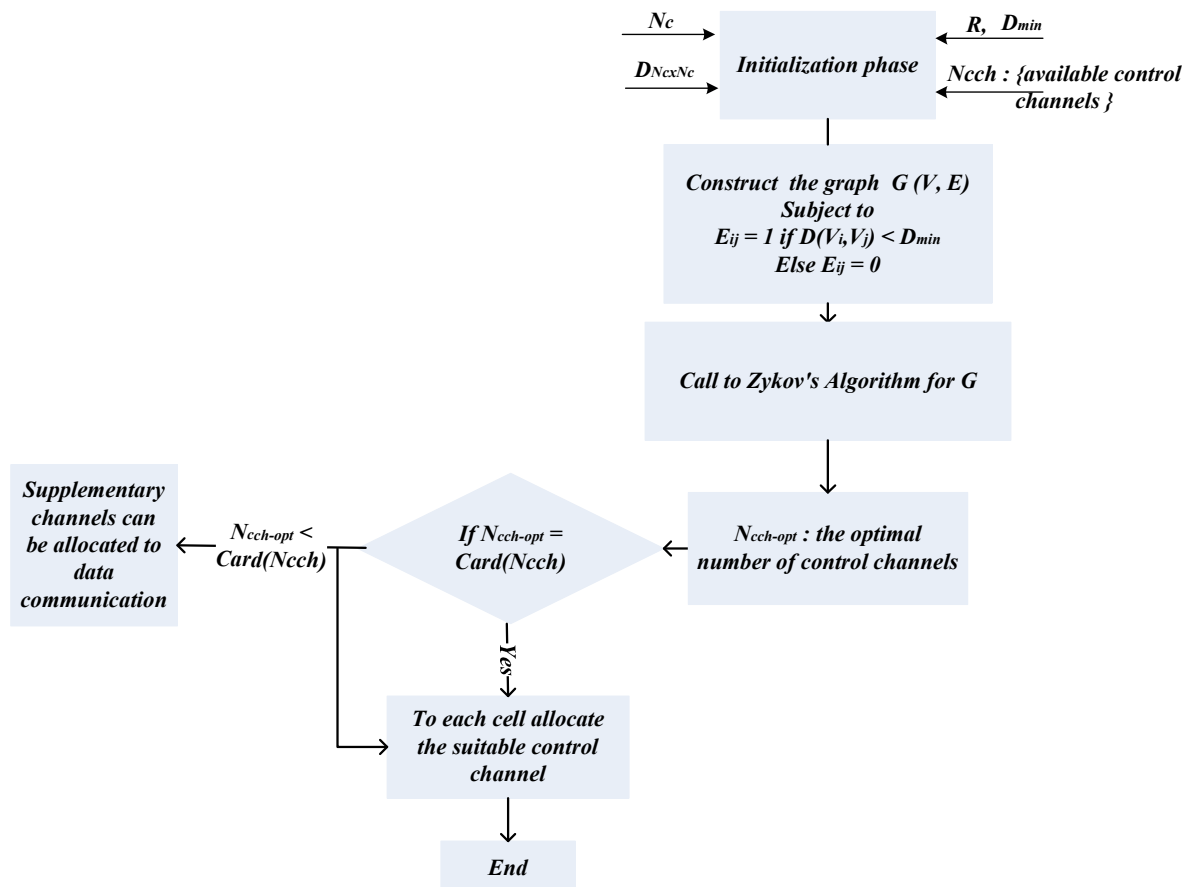
Figure .6: Logical control channel allocation algorithm
