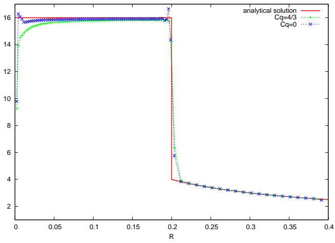
Figure 19: Density as a function of radius for the Noh problem at stopping time t = 0.6 . \Gamma_c = \frac{\gamma+1}{2} computation versus \Gamma_c = 0 computation.
