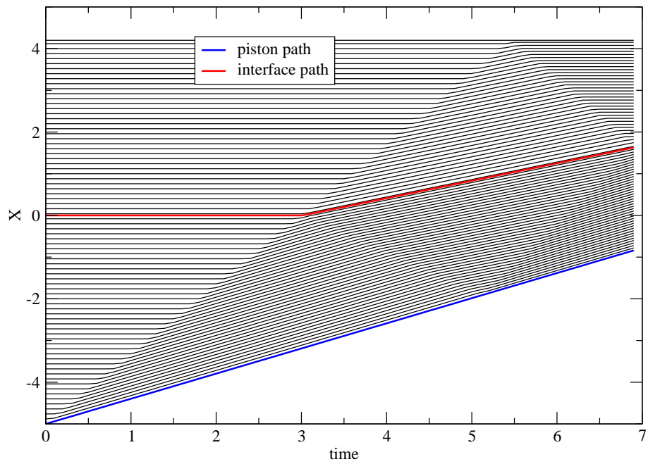
Figure 30: t-x diagram for the shock-contact interaction problem.
