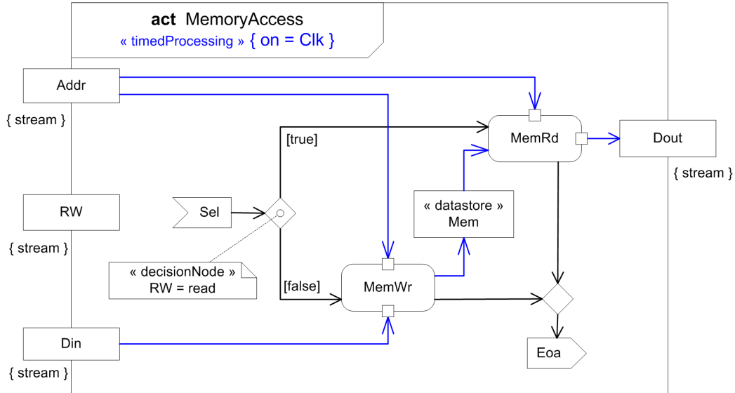
Figure 9: UML Activity for a memory with MARTE annotations.
