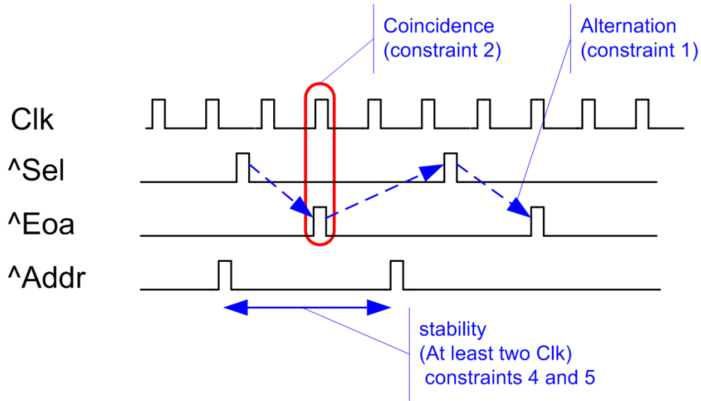
Figure 11: CCSL simulation waveform.
