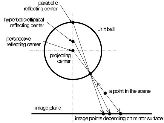
Figure 2. Omni-camera Model.
