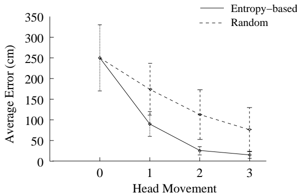
Figure 5: Evolution of the average error (and the standard deviation) w.r.t. the correct position as we get new images.
