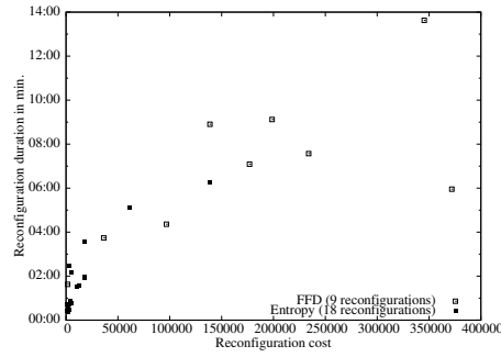
Figure 13: Reconfiguration plans computed by FFD and Entropy
