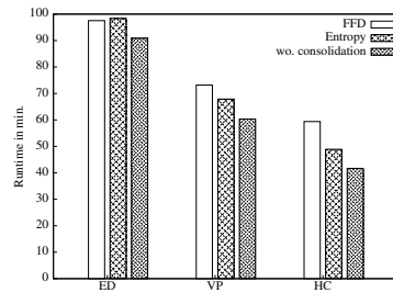
Figure 16: Runtime Comparison
