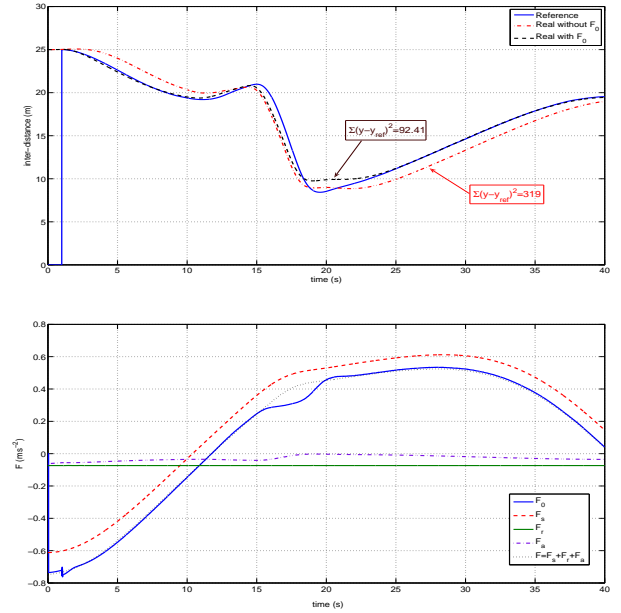
Fig. 5. (a) Inter-distance evolution with and without F estimation. (b) Comparison between real F and its estimate F_0 . Aerodynamic ( F_d ), road slope ( F_s ) and rolling resistance ( F_r ) terms are also depicted.
