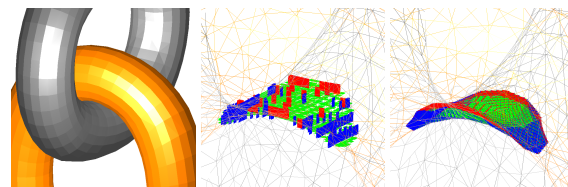
Figure 10: Intersection volume at different resolutions. Left: the collision surfaces. Middle: the intersection volume at resolution 16 \times 16 . Red, green and blue pixel show the bounds in x , y and z directions, respectively. Right: resolution 256 \times 256 .
