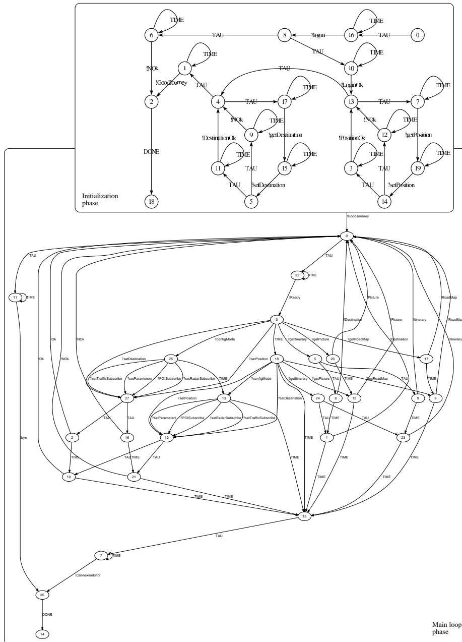
Fig. 4. DTLTS model of the GPS Web service, with zoom on the initialization phase. The action !GoodJourney makes the link between the initialization phase and the main loop phase.
