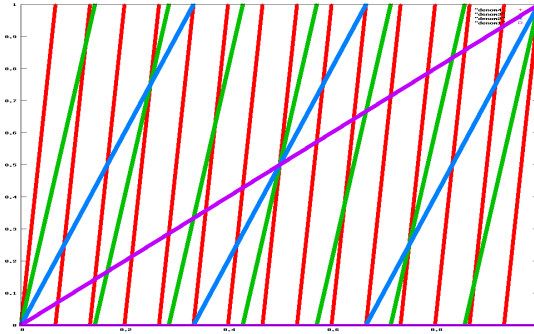
Figure 13: Lines \phi = (2^n - 1)\alpha - i for n \geq 0 and 0 \leq i < 2^n - 1
